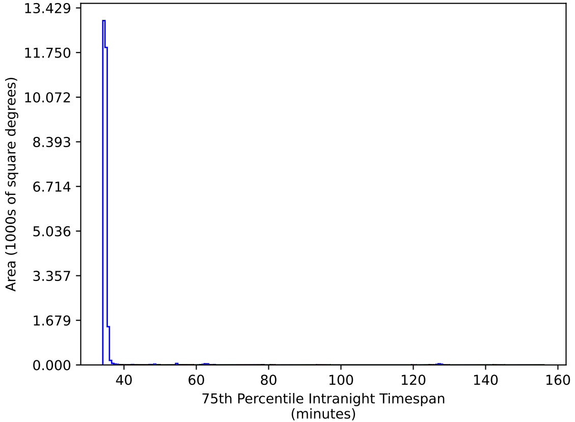
too_combined_s0.5_v3.4_10yrs All sky iz bands: 75th Percentile Intranight Timespan
