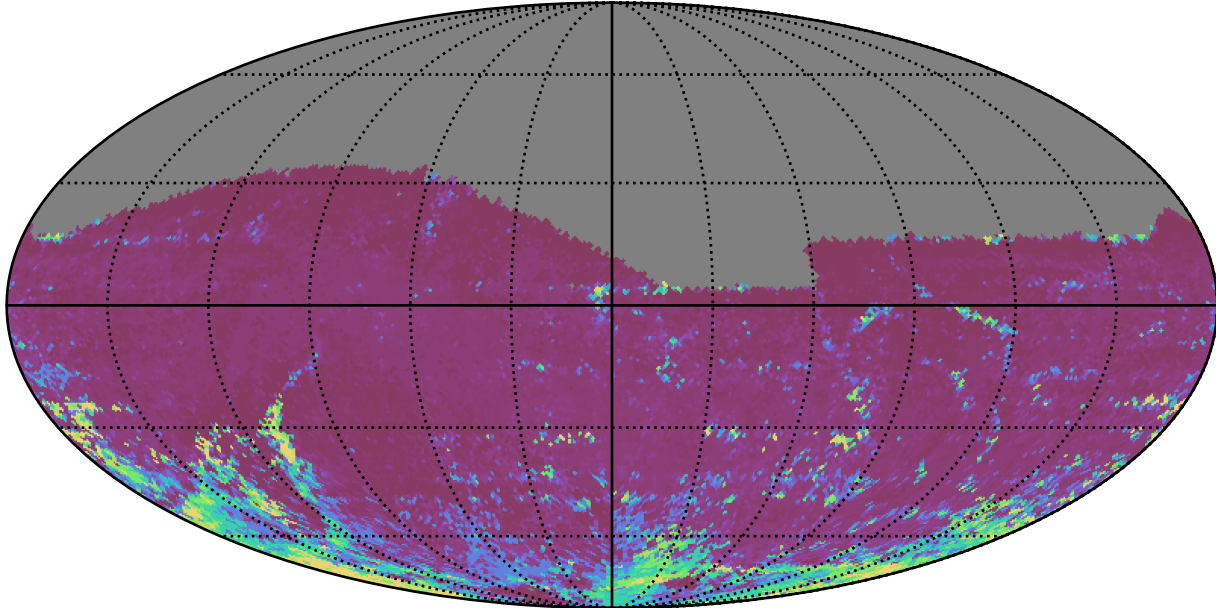
too_combined_s0.5_v3.4_10yrs All sky i band: 75th Percentile Intranight Timespan
