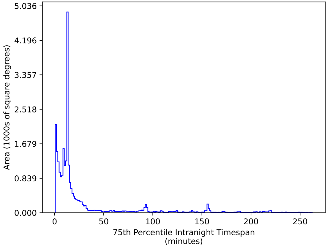
too_combined_s0.5_v3.4_10yrs All sky i band: 75th Percentile Intranight Timespan
