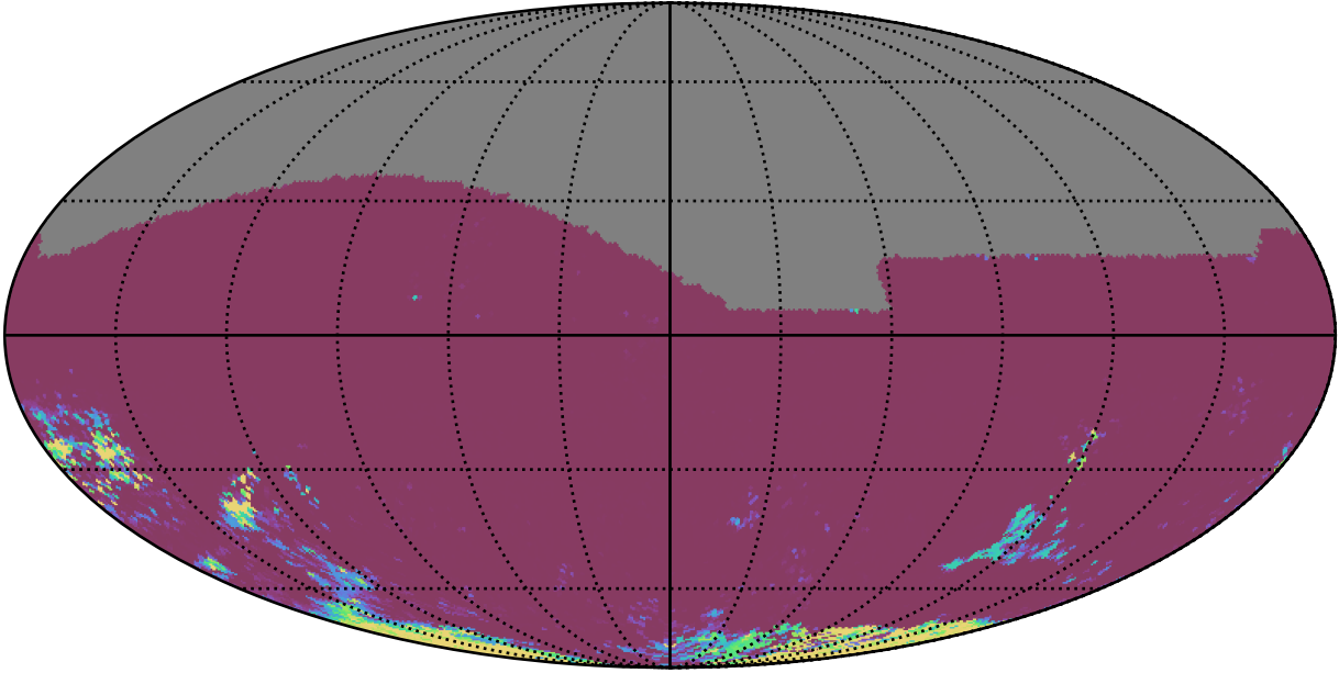
too_combined_s0.5_v3.4_10yrs All sky gr bands: 75th Percentile Intranight Timespan
