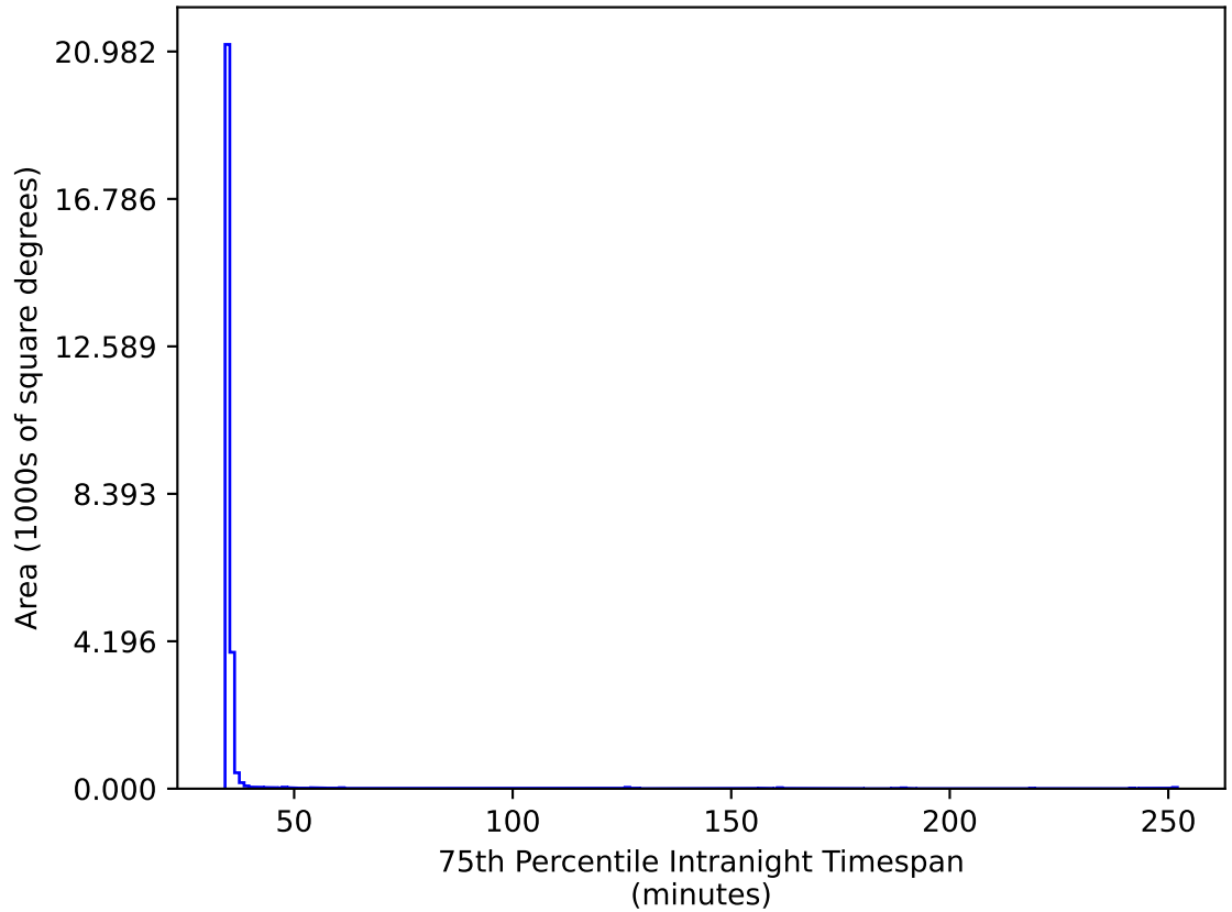
too_combined_s0.5_v3.4_10yrs All sky gr bands: 75th Percentile Intranight Timespan
