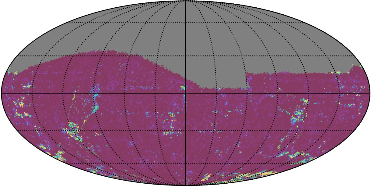
too_combined_s0.5_v3.4_10yrs All sky g band: 75th Percentile Intranight Timespan
