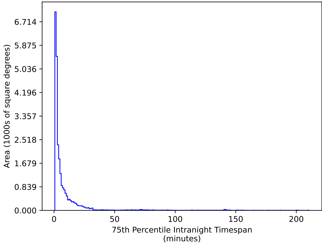
too_combined_s0.5_v3.4_10yrs All sky g band: 75th Percentile Intranight Timespan
