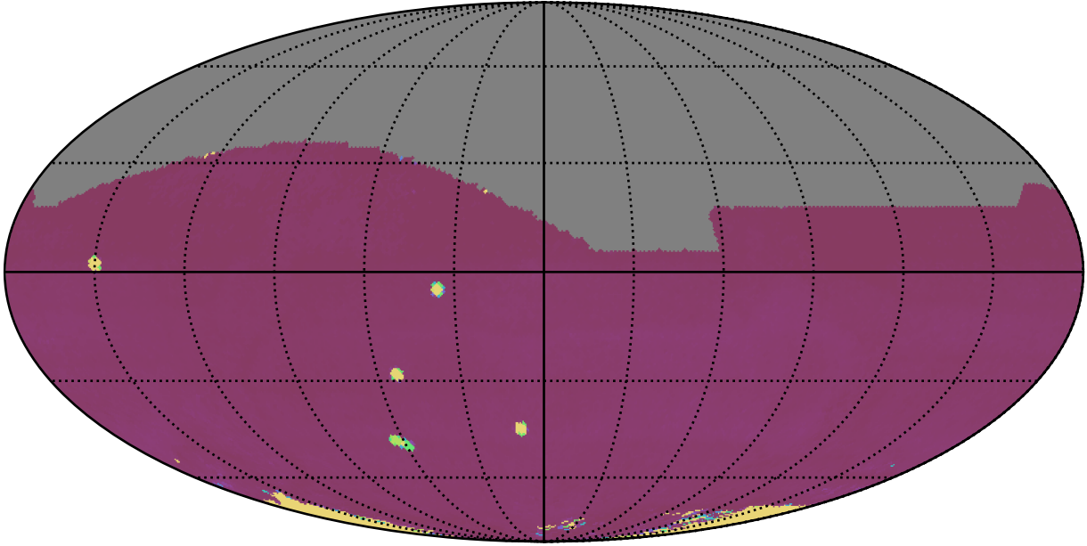
too_combined_s0.5_v3.4_10yrs All sky all bands: 75th Percentile Intranight Timespan
