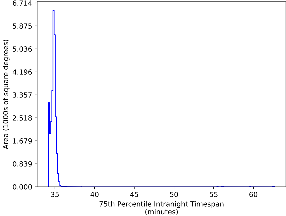
too_combined_s0.5_v3.4_10yrs All sky all bands: 75th Percentile Intranight Timespan
