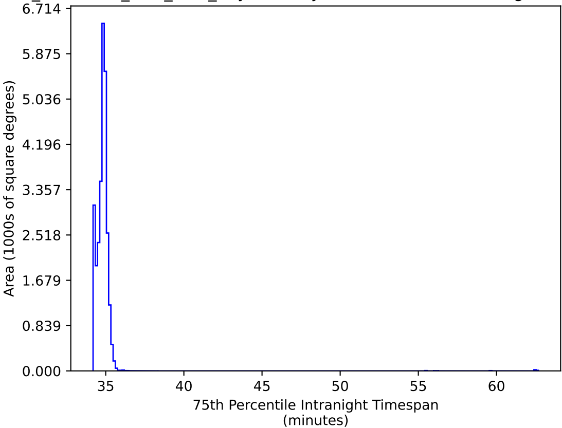
too_combined_s0.5_v3.4_10yrs All sky: 75th Percentile Intranight Timespan
