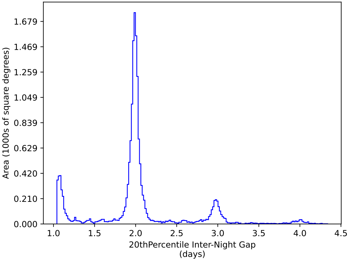
too_combined_s0.5_v3.4_10yrs WFD y band: 20thPercentile Inter-Night Gap
