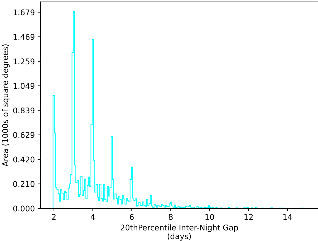
too_combined_s0.5_v3.4_10yrs WFD u band: 20thPercentile Inter-Night Gap
