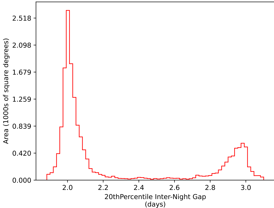
too_combined_s0.5_v3.4_10yrs WFD i band: 20thPercentile Inter-Night Gap
