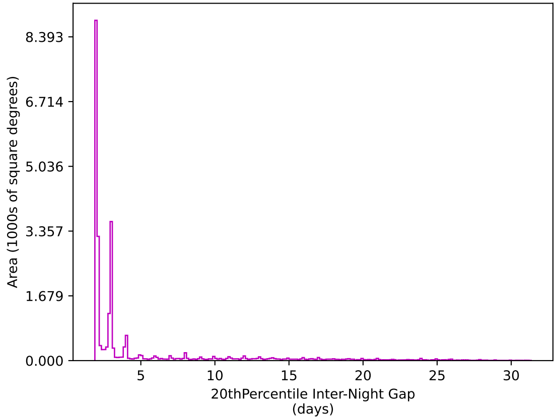
too_combined_s0.5_v3.4_10yrs All sky z band: 20thPercentile Inter-Night Gap
