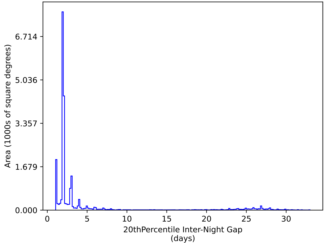
too_combined_s0.5_v3.4_10yrs All sky y band: 20thPercentile Inter-Night Gap
