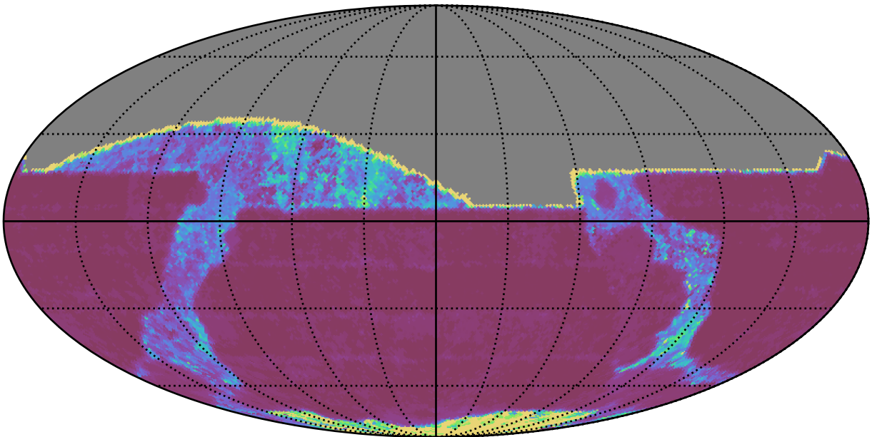
too_combined_s0.5_v3.4_10yrs All sky i band: 20thPercentile Inter-Night Gap
