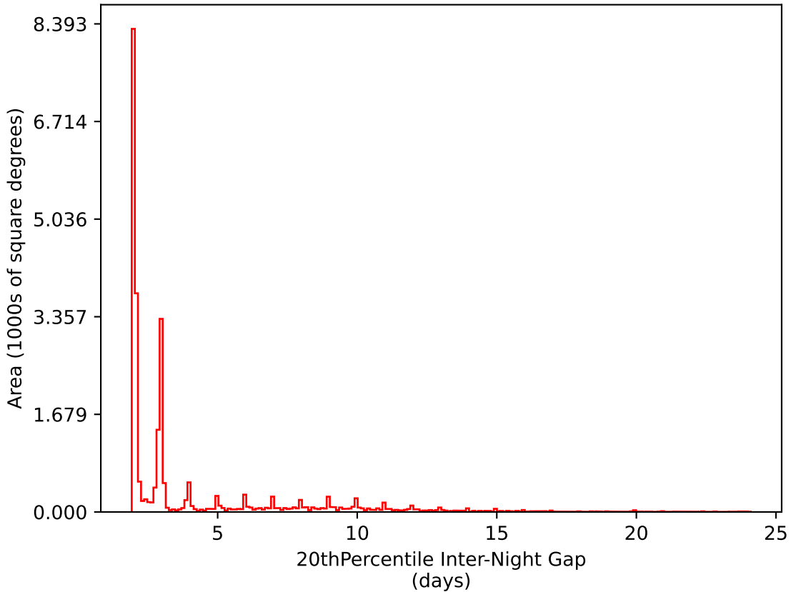
too_combined_s0.5_v3.4_10yrs All sky i band: 20thPercentile Inter-Night Gap
