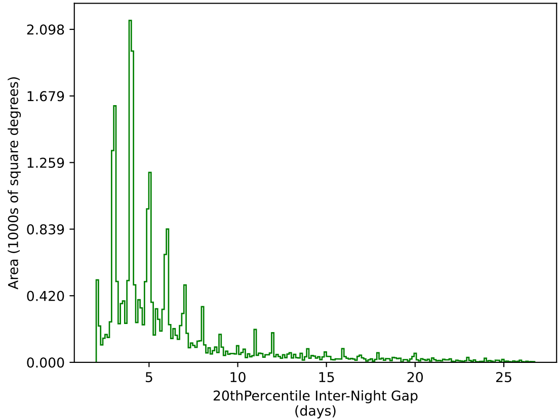
too_combined_s0.5_v3.4_10yrs All sky g band: 20thPercentile Inter-Night Gap
