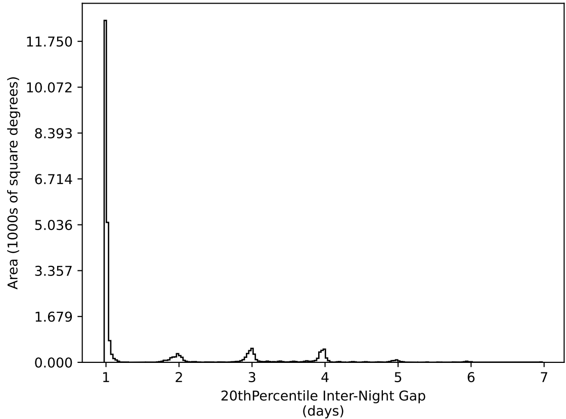
too_combined_s0.5_v3.4_10yrs All sky all bands: 20thPercentile Inter-Night Gap
