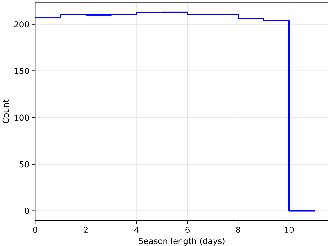
too_combined_s0.5_v3.4_10yrs DD:EDFS all bands: SeasonLength
