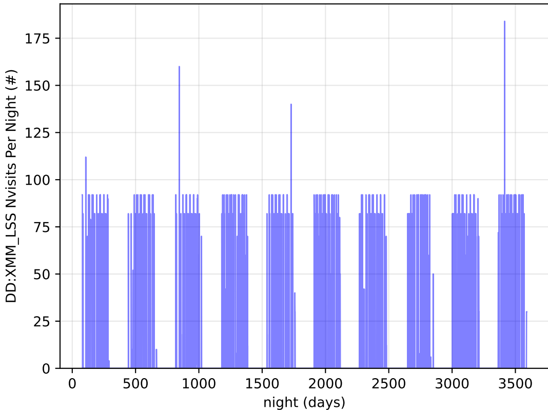
too_combined_s0.5_v3.4_10yrs all bands: DD:XMM_LSS Nvisits Per Night
