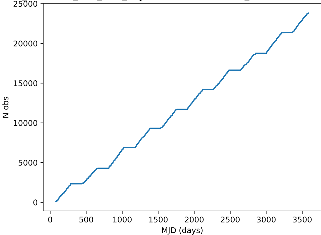
too_combined_s0.5_v3.4_10yrs all bands: DD:XMM_LSS Cumulative NVisits
