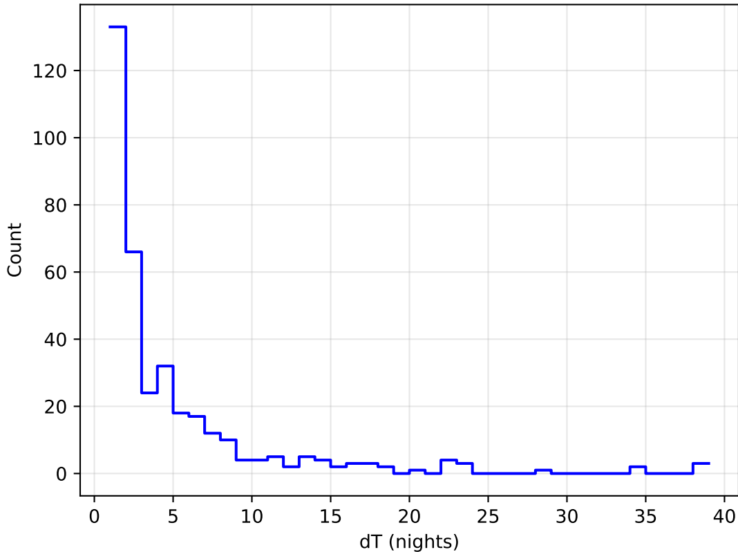
too_combined_s0.5_v3.4_10yrs all bands: DD:WFD Delta Nights Histogram
