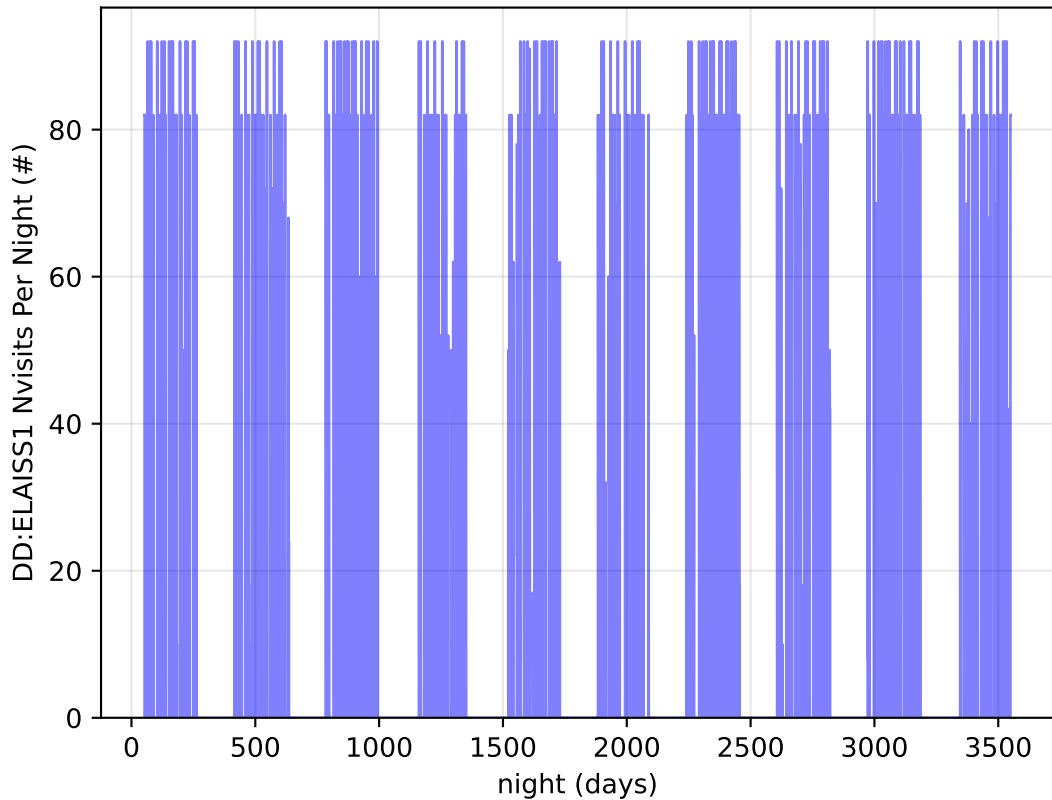
too_combined_s0.5_v3.4_10yrs all bands: DD:ELAISS1 Nvisits Per Night
