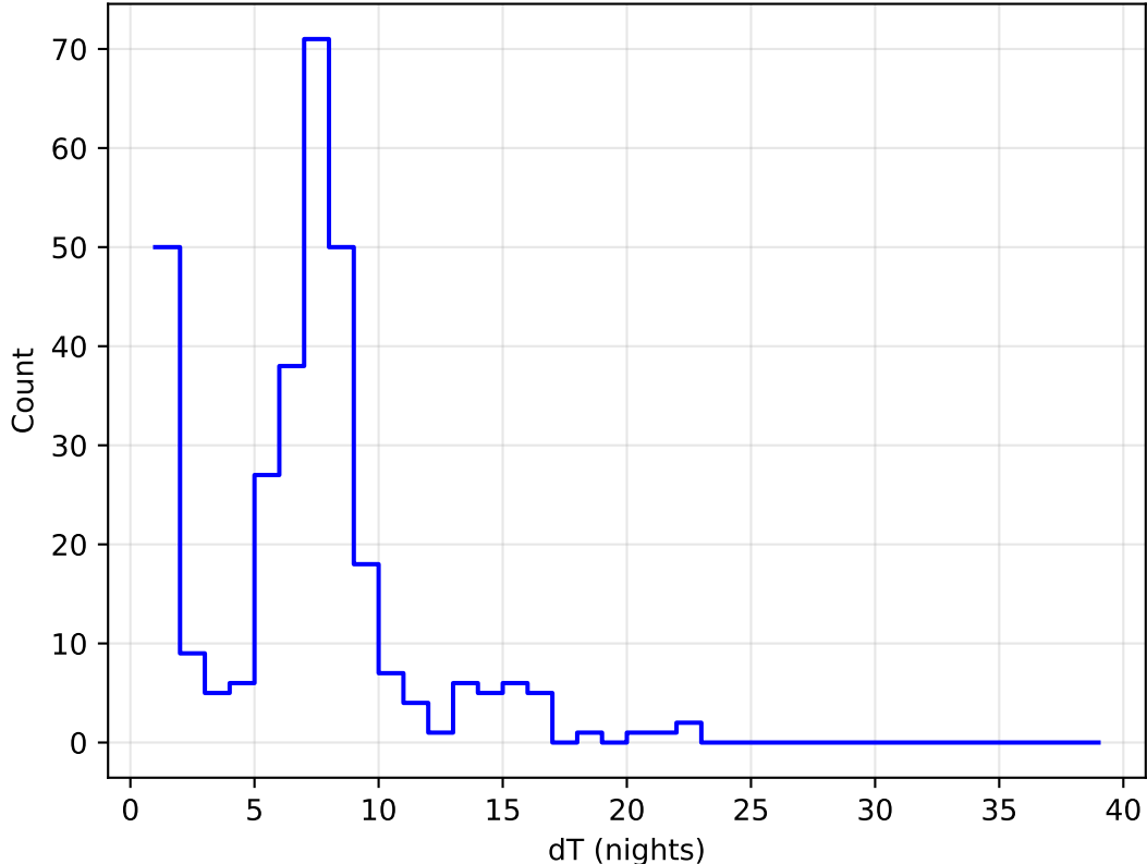
too_combined_s0.5_v3.4_10yrs all bands: DD:ELAISS1 Delta Nights Histogram
