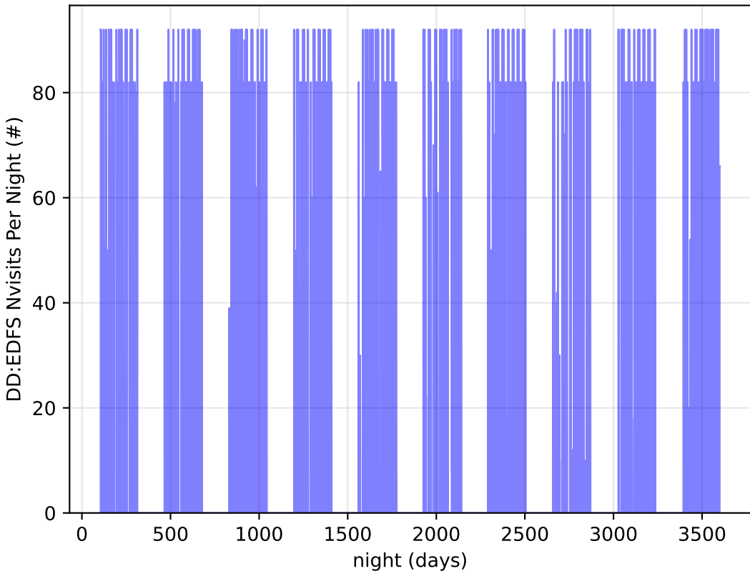
too_combined_s0.5_v3.4_10yrs all bands: DD:EDFS Nvisits Per Night
