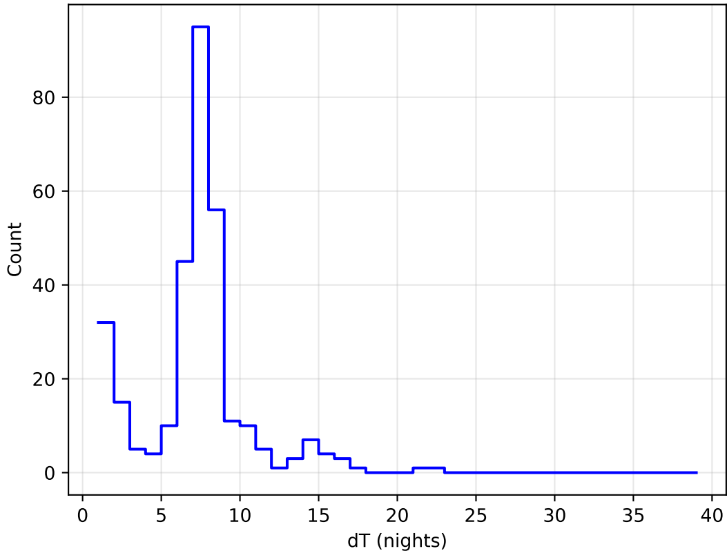
too_combined_s0.5_v3.4_10yrs all bands: DD:EDFS Delta Nights Histogram
