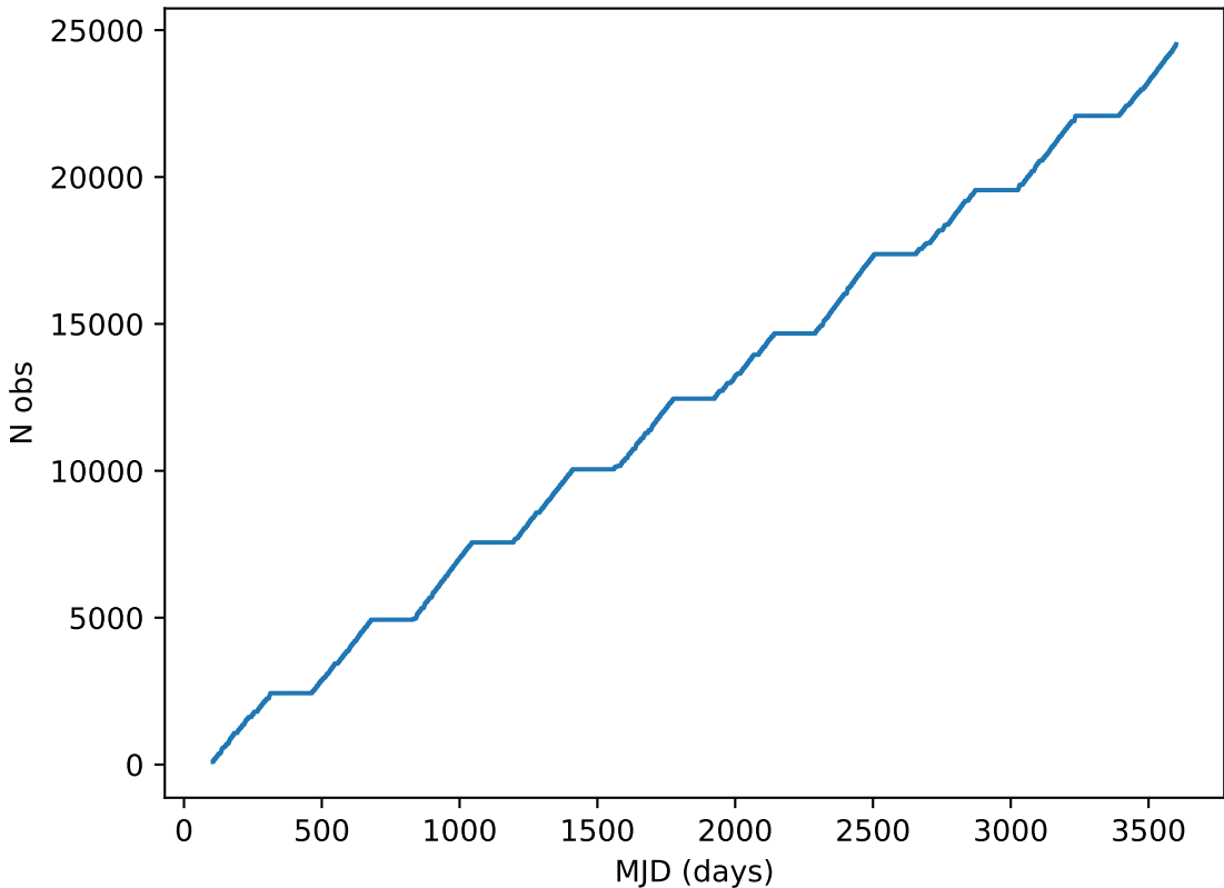
too_combined_s0.5_v3.4_10yrs all bands: DD:EDFS Cumulative NVisits
