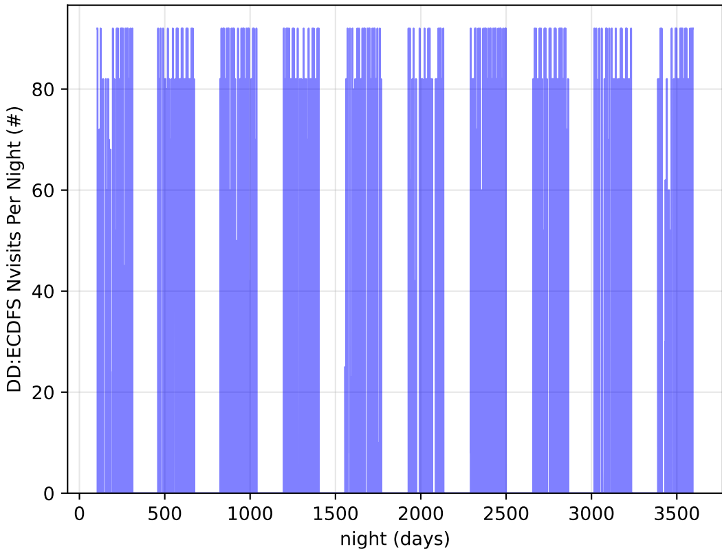
too_combined_s0.5_v3.4_10yrs all bands: DD:ECDFS Nvisits Per Night
