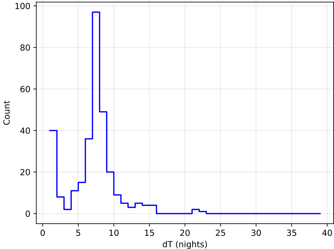
too_combined_s0.5_v3.4_10yrs all bands: DD:ECDFS Delta Nights Histogram
