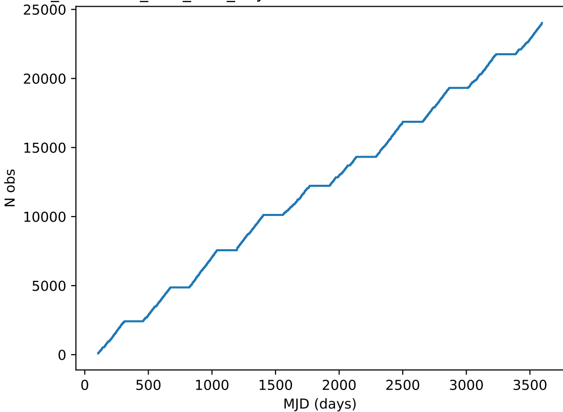
too_combined_s0.5_v3.4_10yrs all bands: DD:ECDFS Cumulative NVisits
