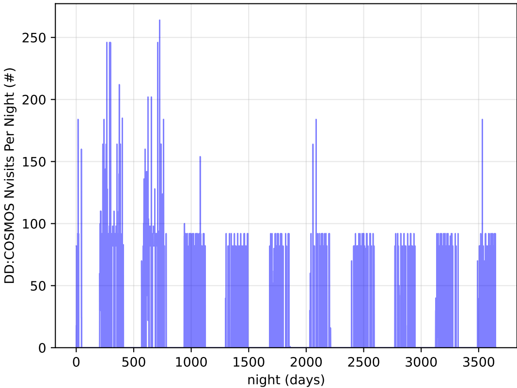
too_combined_s0.5_v3.4_10yrs all bands: DD:COSMOS Nvisits Per Night
