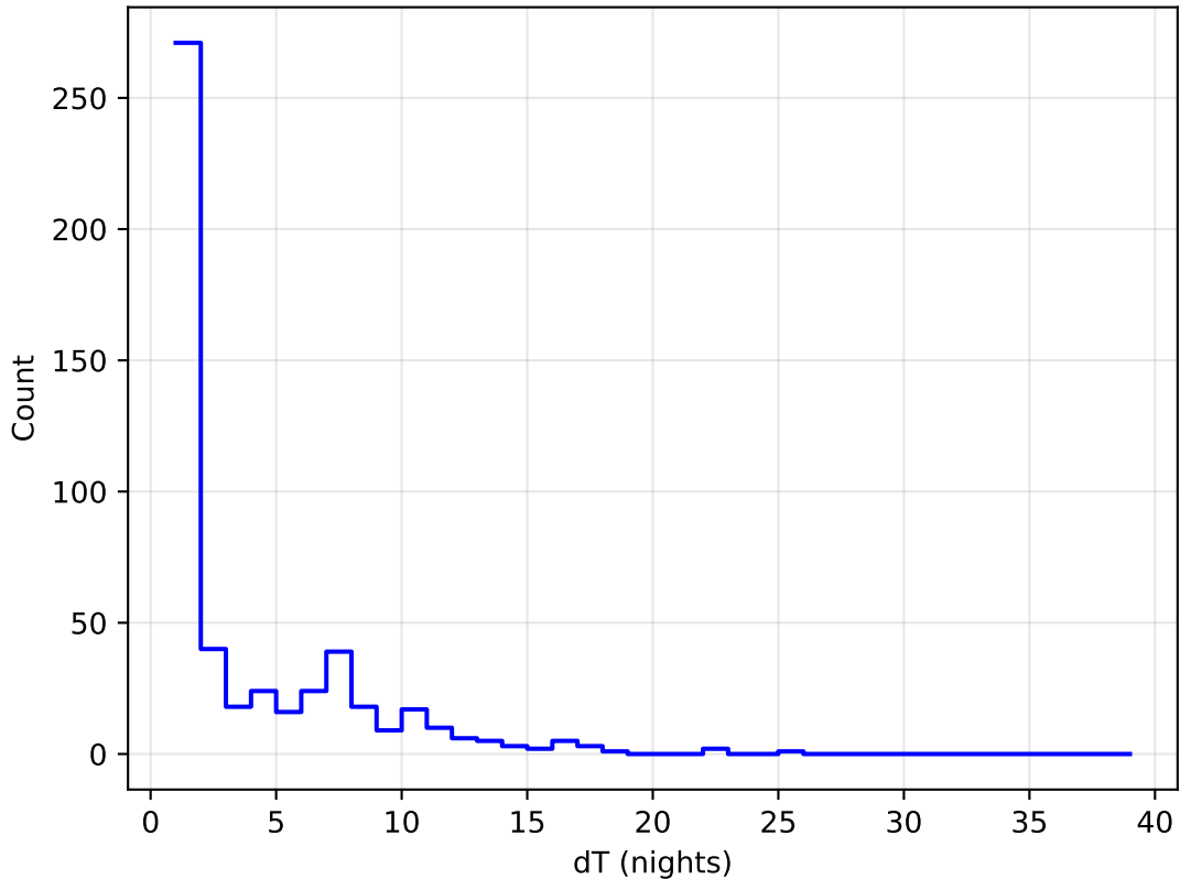
too_combined_s0.5_v3.4_10yrs all bands: DD: COSMOS Delta Nights Histogram
