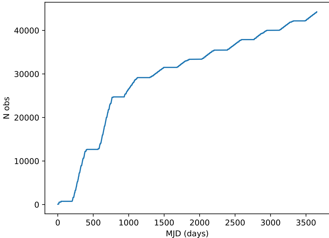
too_combined_s0.5_v3.4_10yrs all bands: DD:COSMOS Cumulative NVisits
