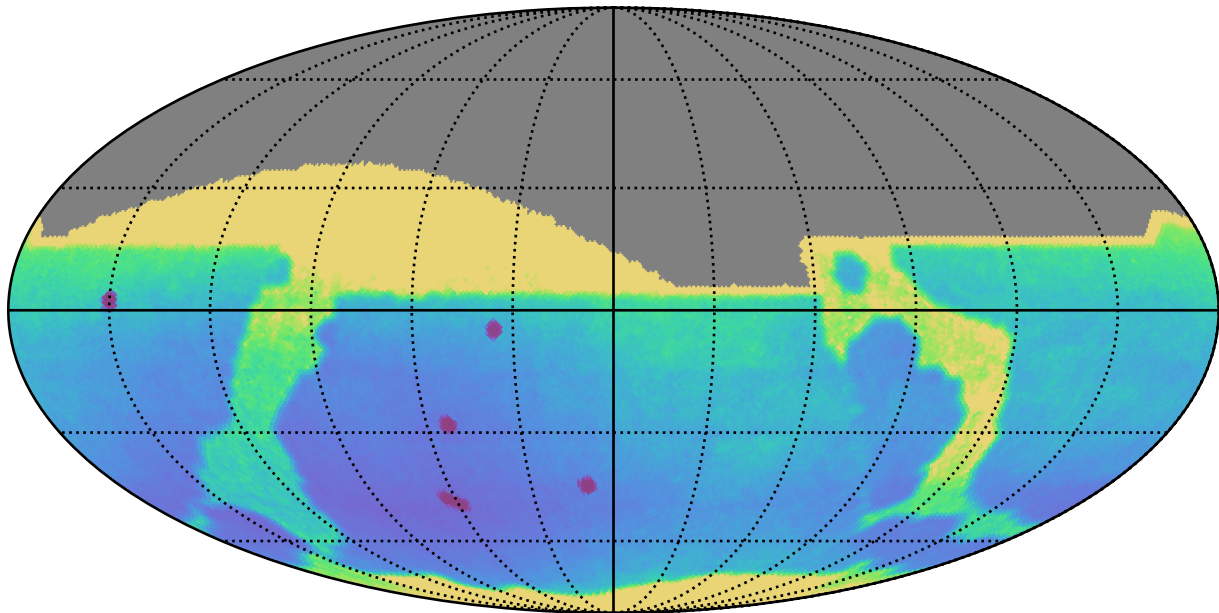
too_combined_s0.0_v3.4_10yrs All sky: Parallax Uncert @ 22.4
