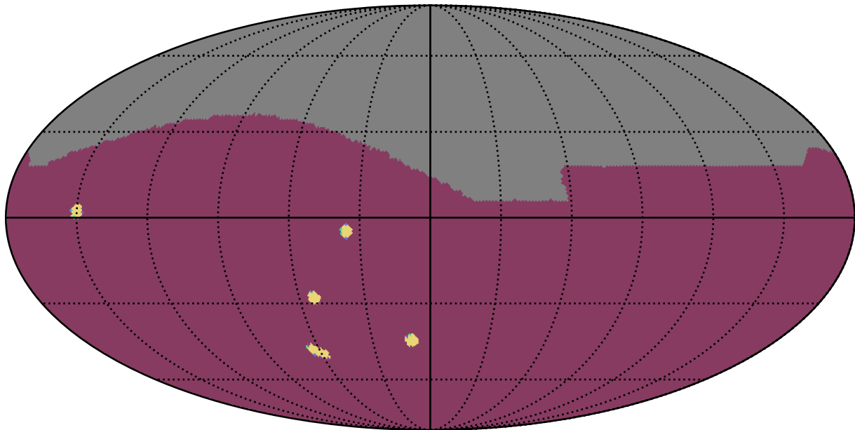
too_combined_s0.0_v3.4_10yrs All sky: NumberOfQuickRevisits
