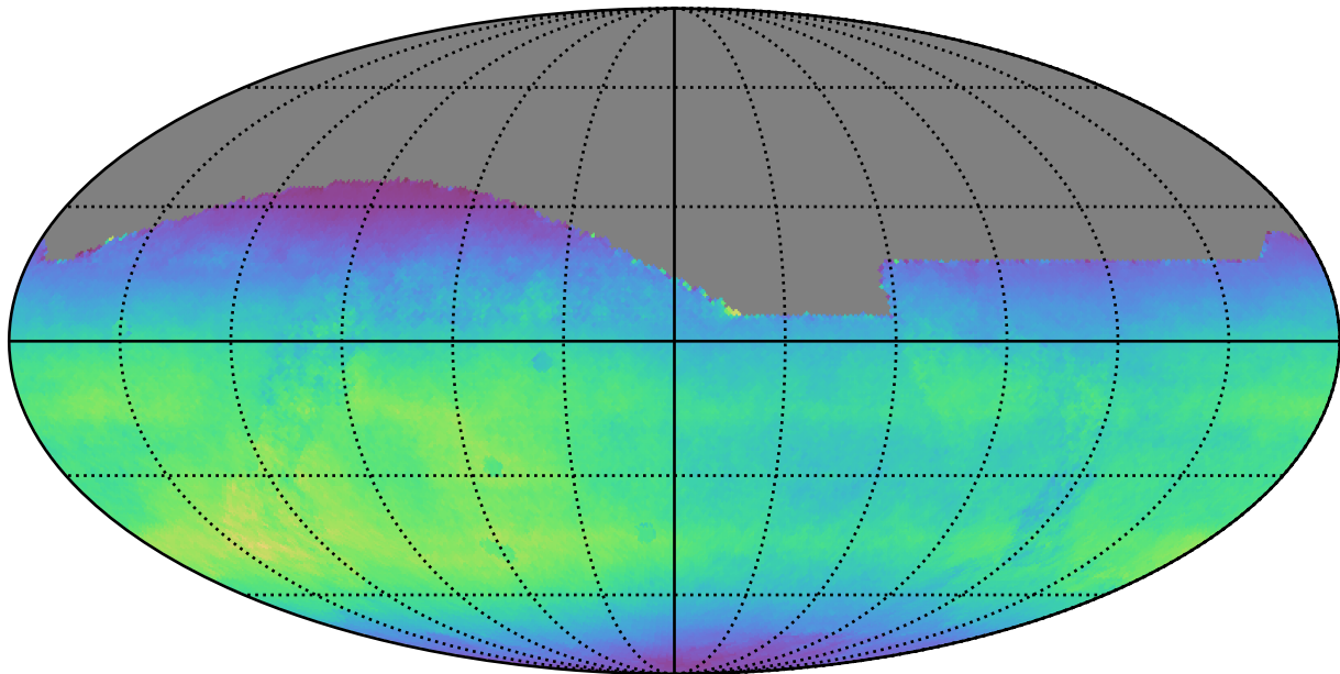
too_combined_s0.0_v3.4_10yrs All sky all bands: Normalized Teff
