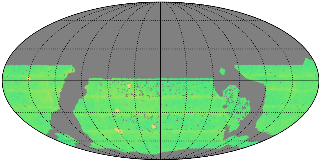
too_combined_s0.0_v3.4_10yrs WFD all bands: N Unique Nights
