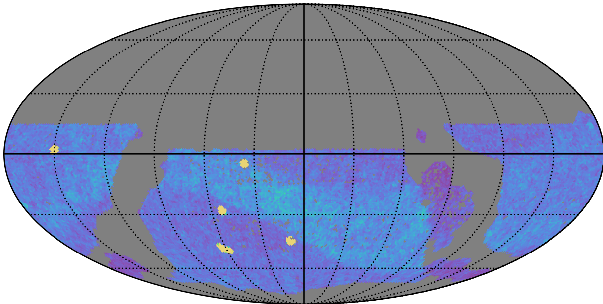
too_combined_s0.0_v3.4_10yrs WFD z band: NVisits
