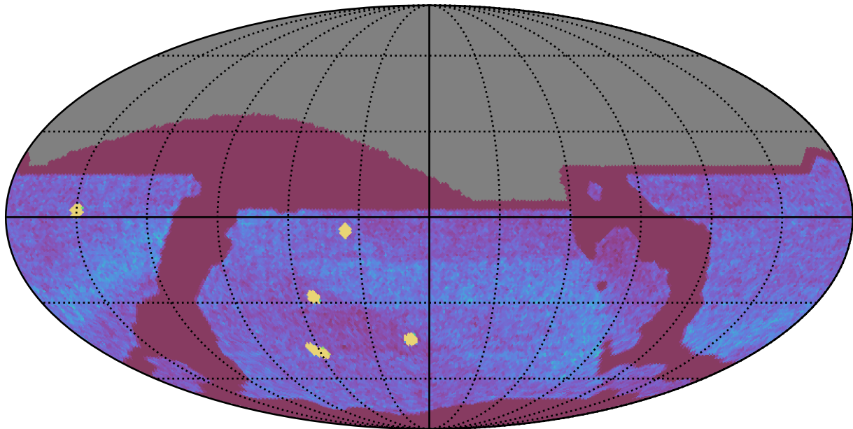
too_combined_s0.0_v3.4_10yrs All sky all bands: NVisits
