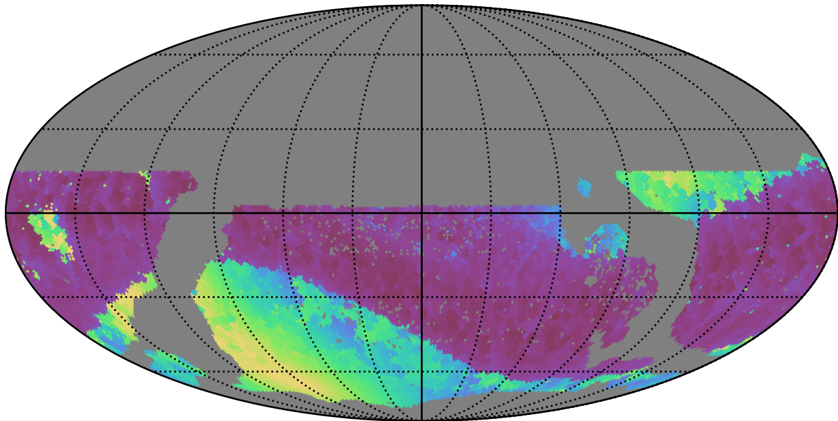
too_combined_s0.0_v3.4_10yrs WFD i band: Min solarElong
