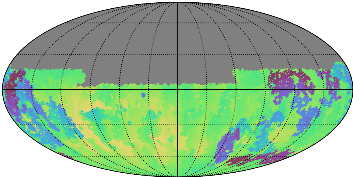
too_combined_s0.0_v3.4_10yrs Yr 1 u band: Min skyBrightness
