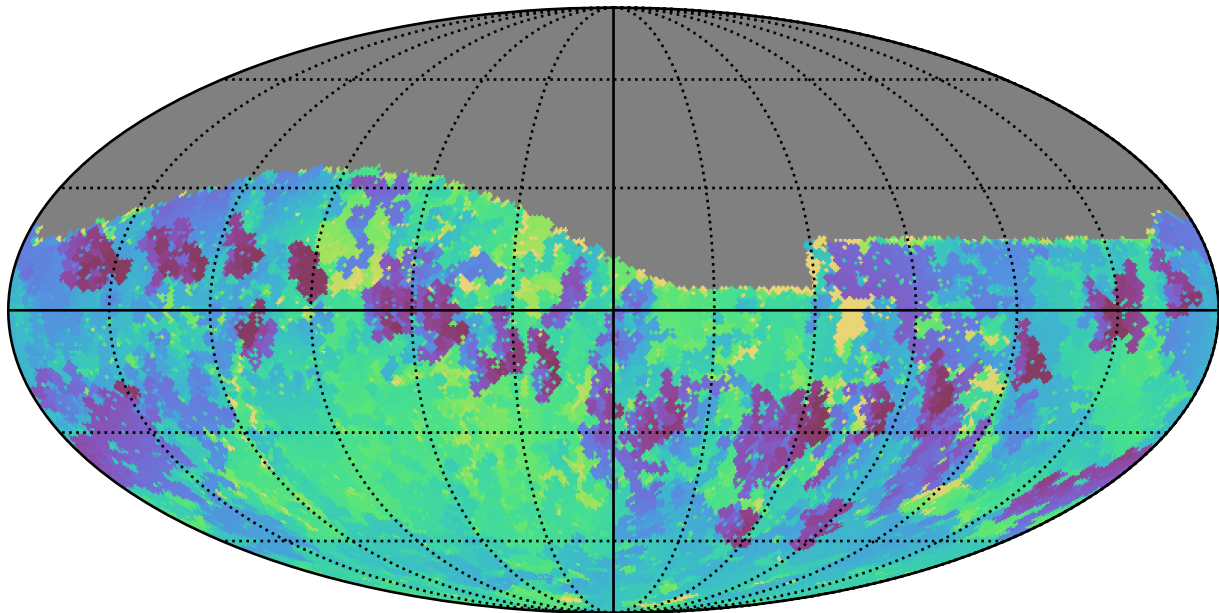
too_combined_s0.0_v3.4_10yrs Yr 1 i band: Min skyBrightness
