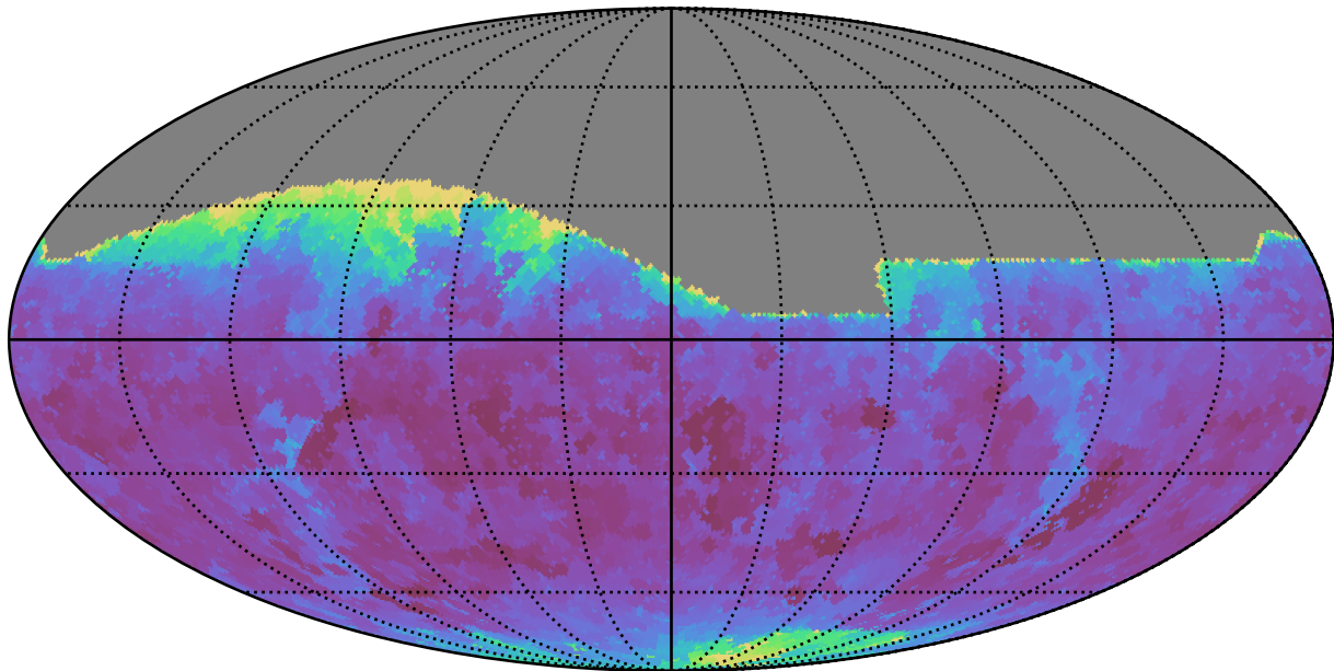
too_combined_s0.0_v3.4_10yrs All sky z band: Min seeingEff
