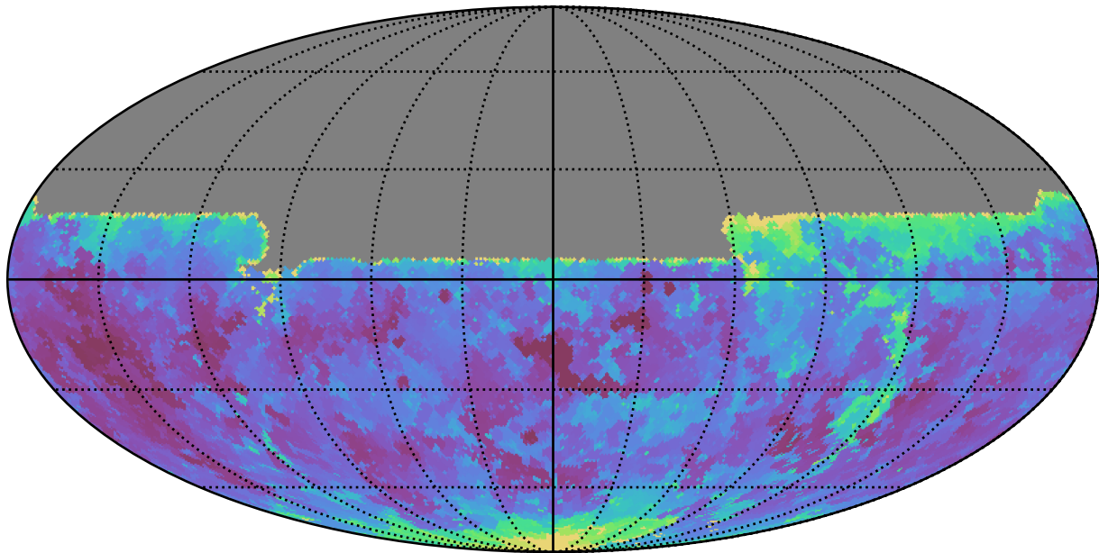
too_combined_s0.0_v3.4_10yrs All sky u band: Min seeingEff
