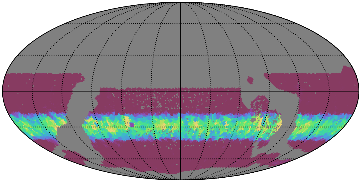
too_combined_s0.0_v3.4_10yrs WFD u band: Min normairmass
