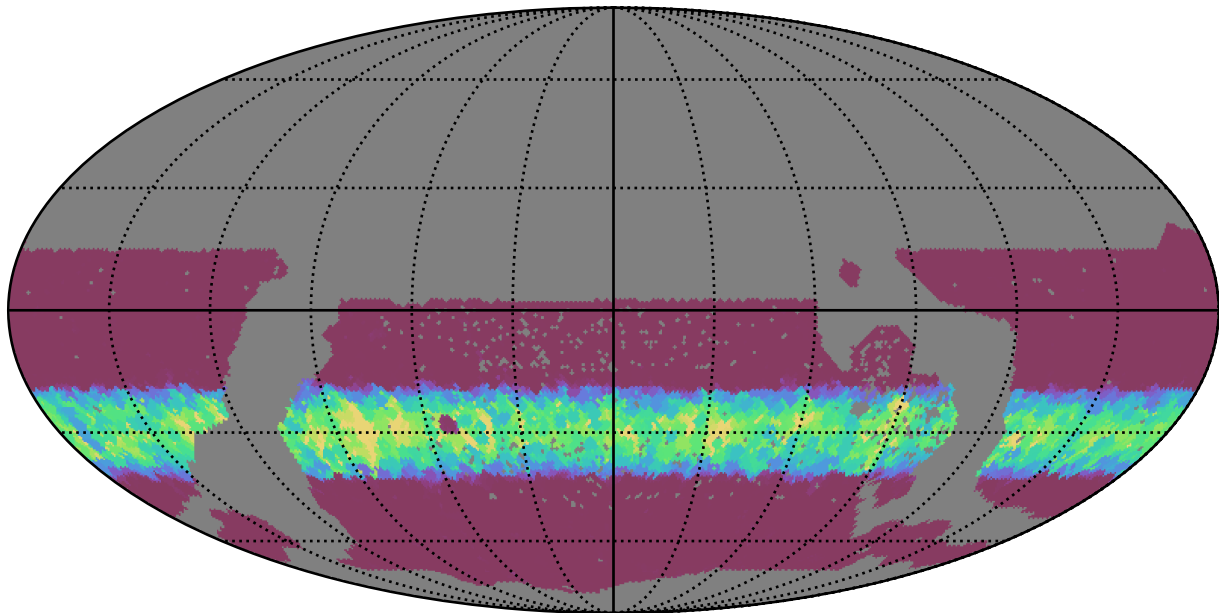
too_combined_s0.0_v3.4_10yrs WFD g band: Min normairmass
