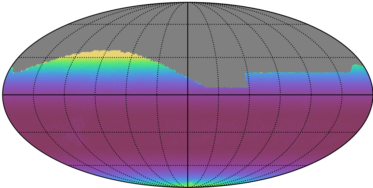
too_combined_s0.0_v3.4_10yrs All sky z band: Min airmass
