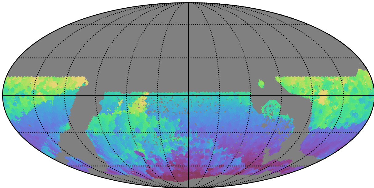
too_combined_s0.0_v3.4_10yrs WFD r band: Min HA
