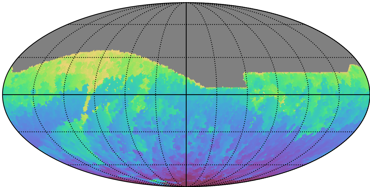
too_combined_s0.0_v3.4_10yrs All sky i band: Min HA
